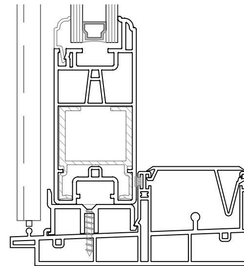
2 Sill Detail
