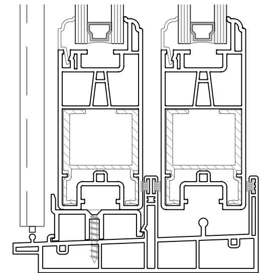
4 Sill Detail
