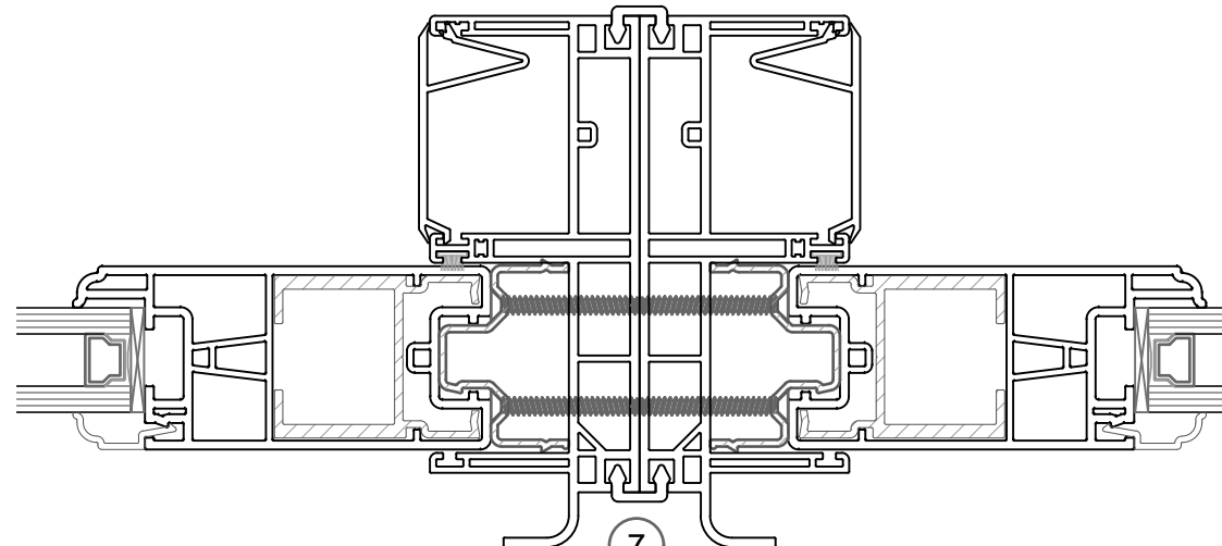
7 Mullion Detail
